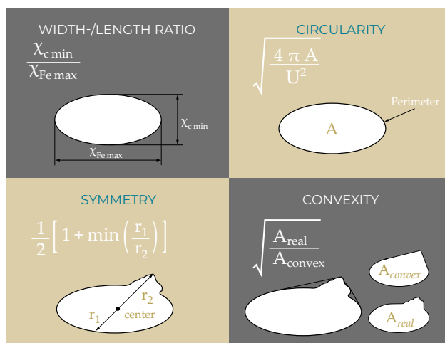
Fig. 2: Selection of basic shape parameters (CAMSIZER X2).
