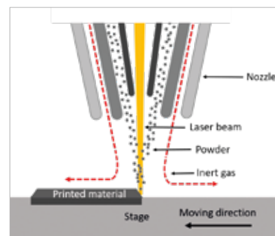
Fig. 1: process of additive laser powder build-up welding.
